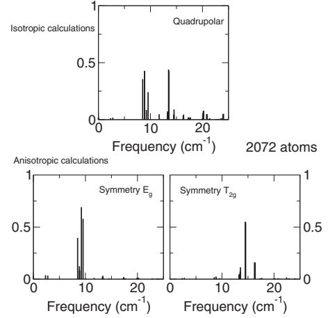
FIG. 1. Projection of the fundamental quadrupolar elastic vibration modes of a 4.3 nm diameter silver spherical NP, calculated using the linear elasticity theory on atomistic ones using the scalar product given in Eqs. (2) and (4). Results are reported for both isotropic (above) and anisotropic (below) calculations. For isotropic calculations, the quadrupolar elastic vibrations modes form a set of five degenerated modes with the same irreducible representations. In the anisotropic calculations, quadrupolar modes splits in two sets of modes of respective symmetry E_g and T_{2g} . Abscissa denotes atomistic modes using their frequency in \text{cm}^{-1} .
