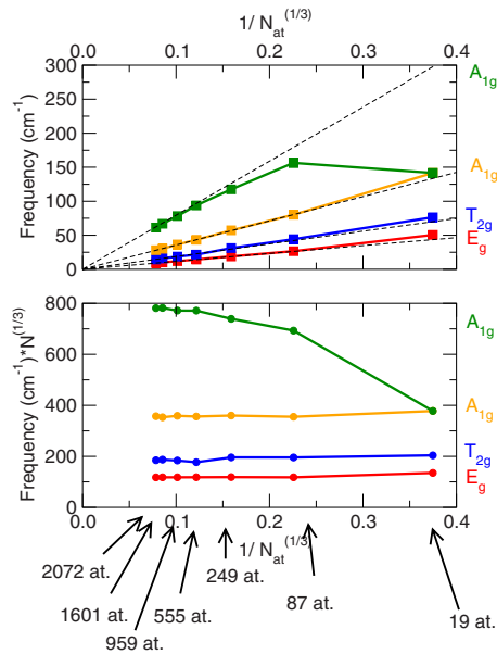
FIG. 4. (Color online) (Above) Frequencies of the atomistic modes onto which the E_g and T_{2g} modes coming from the fundamental quadrupolar modes and the A_{1g} modes coming from the fundamental (low frequency) and first overtone (high frequency) of the breathing mode preferentially project in spherical silver NPs as a function of the inverse of the number of atoms at the power one third. Dashed lines correspond to frequencies calculated by the elasticity theory; the number of atoms is calculated from the ratio of the NP volume on the atomic volume computed from atomistic calculations. (Below) Product of the frequency and the number of atoms at the power one third as a function of the inverse of the number of atoms at the power one third. Linear elasticity predicts horizontal straight lines.
